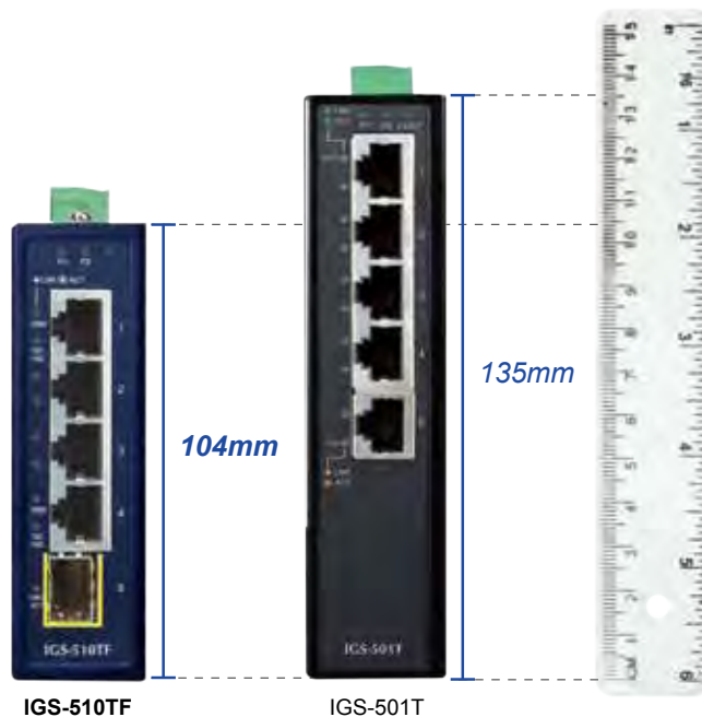
Compact Industrial 5-Port Switch
