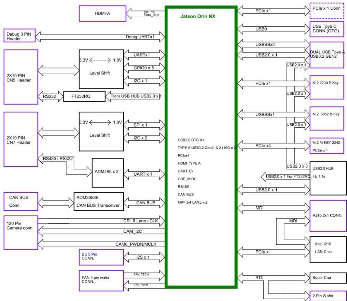
AIB-MO22/32 & AIB-MN32/42 Block diagram
