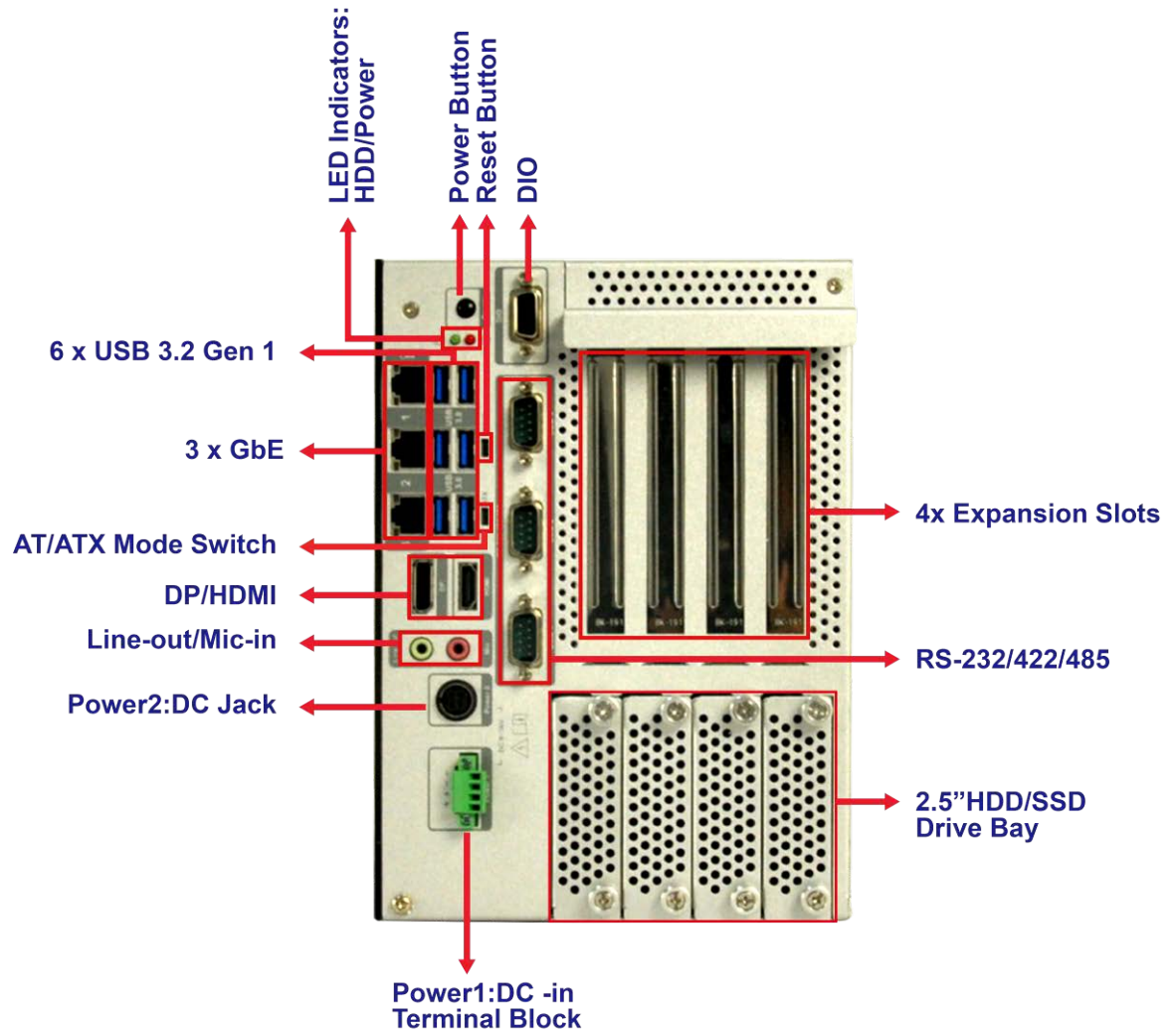
Figure 1-2: Front Panel
