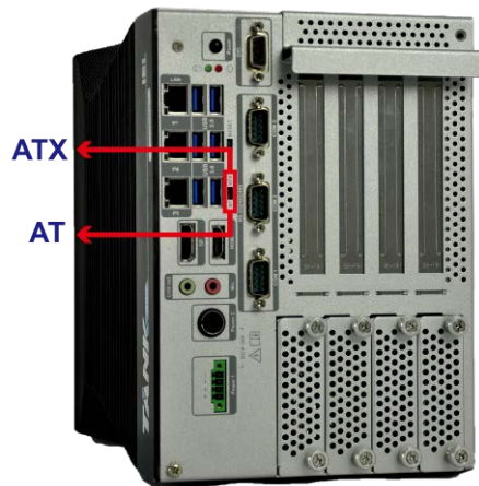
Figure 3-7: AT/ATX Power Mode Switch
