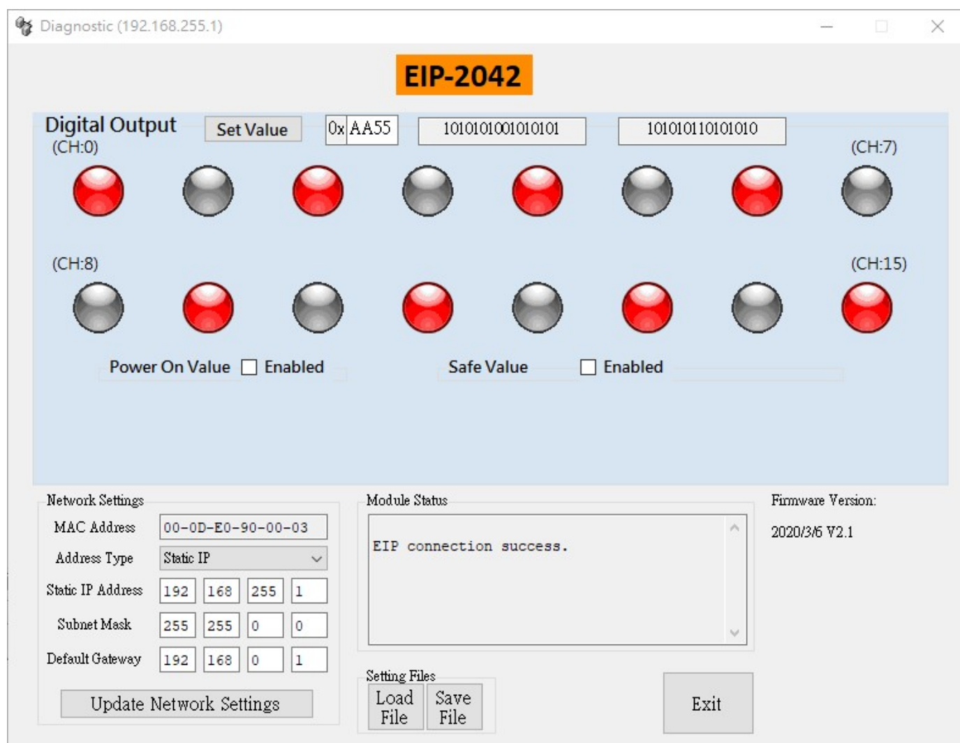
Figure3-3. the steps to test EIP-2000 Utility of DIO module
