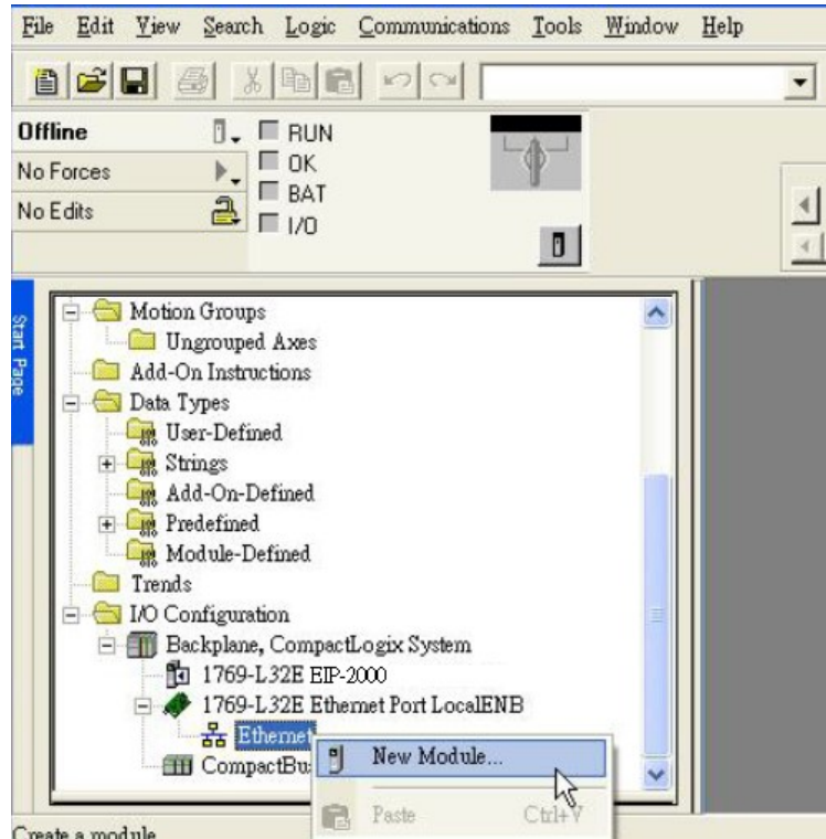
Figure 7-3. Create a new module.
