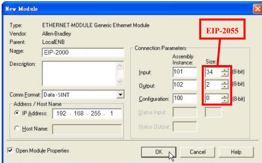
Figure7-5. The settings of EIP-2055
