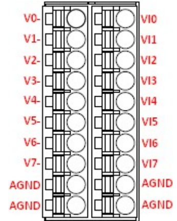
Spring-type terminal connector
