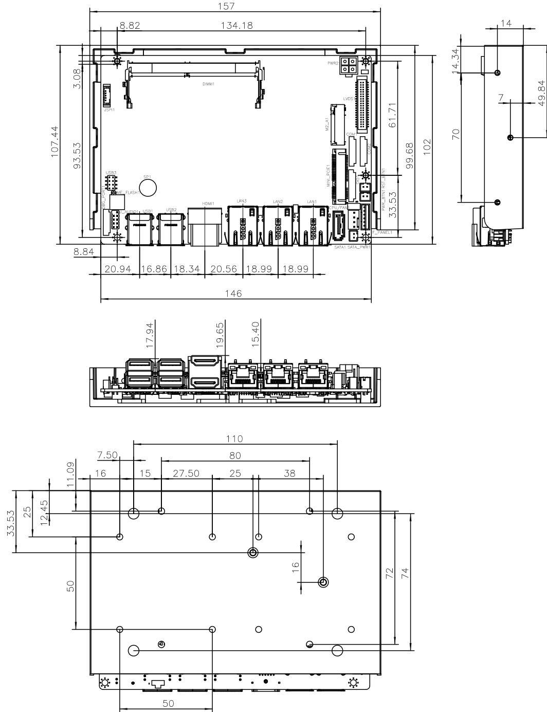
Figure 1-3: Dimensions (mm)
